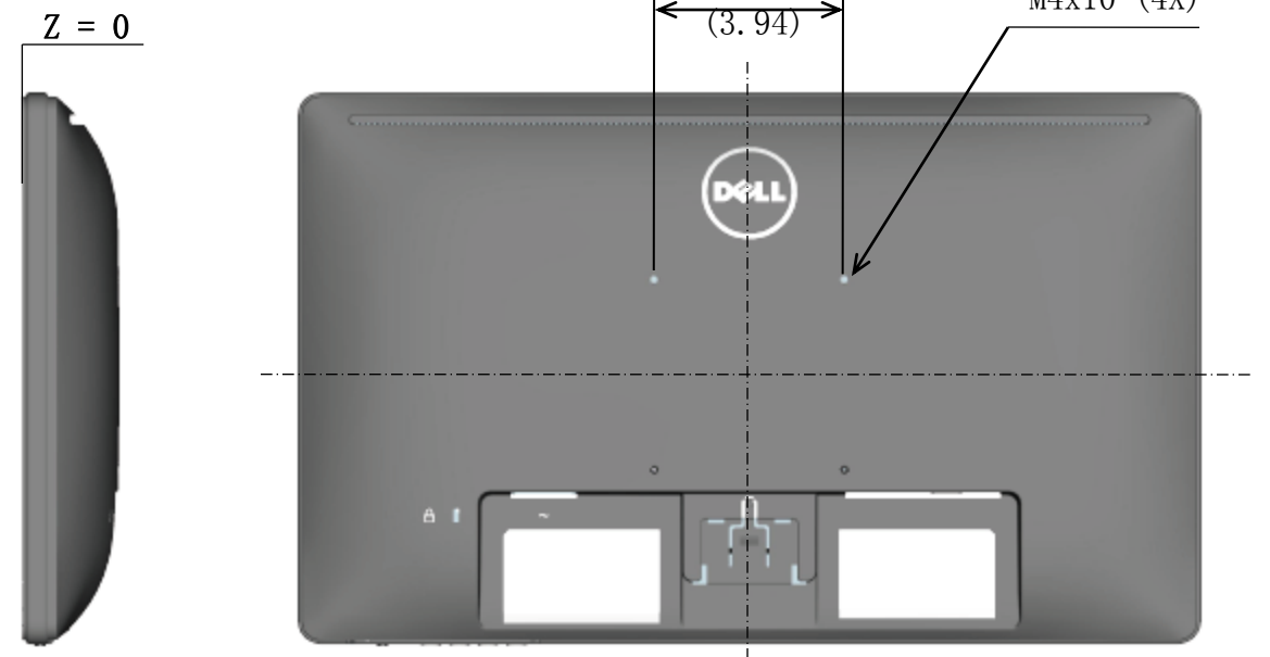
Back view of Monitor without stand
